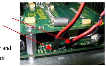
Fig. 3.6.2g Top View: 6KPM Module installed and insight for connecting two wires to the right pins
